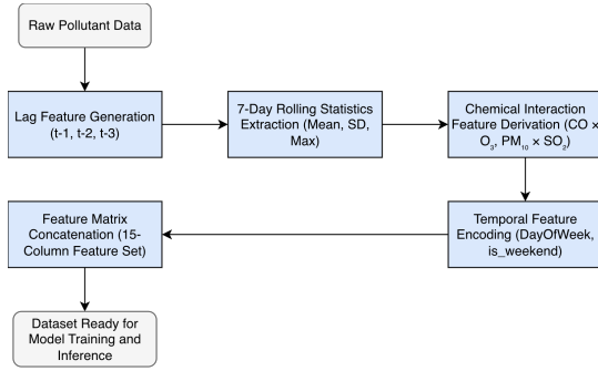
Figure 2: Algorithmic pipeline for multi-variate transformation, lag extraction, and composite chemical interaction generation.
