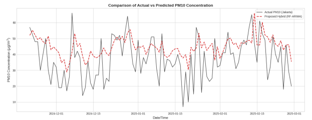
Figure 4: Chronological forecasting path tracking actual PM_{10} fluctuations versus sequential hybrid model tracking curves.
