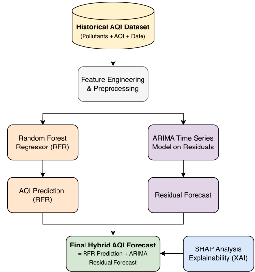
Figure 3: Sequential hybrid architecture block diagram detailing the segregation of non-linear patterns and linear residual auto-correlations.
