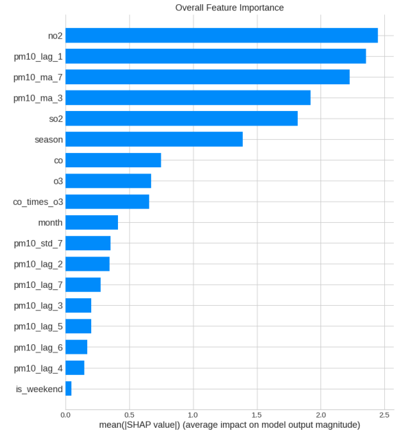
Figure 7: Global feature importance ranking mapped via average absolute Shapley values ( TreeSHAP ).
