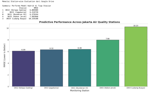
Figure 5: Multi-station spatial evaluation metrics mapping localized validation deviations across Jakarta SPKUA networks.
